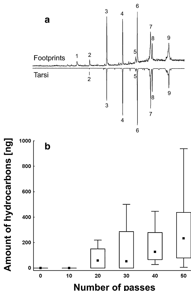
Fig. 2 a Ion chromatograms of hexane wash of microscopic slide that was walked over 50 times by Bombus terrestris workers in the nest entrance tunnel (top) and hexane extract of the tarsi of an individual worker (bottom). Peak assignment: 1 contamination, 2 heneicosane, 3 tricosane, 4 pentacosane, 5 heptacosene, 6 heptacosane, 7 nonacosene, 8 nonacosane, 9 untriacontene (ISTD internal standard). b Amount of total hydrocarbons in microscopic slide washes in relation to the number of times the slides were passed by bees in the nest entrance tunnel (median, quartile range, and non-outlier range)
