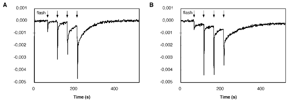
FIG. 4. P_{700} turnover kinetics of PS I. Wild-type (A) and petM - strains (B) show the same kinetics of re-reduction. Identical chlorophyll concentrations were used for both types of cells, which were flashed four times with far red light while absorbance changes were monitored at 703 nm.
