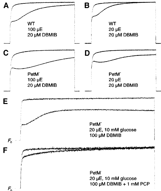
FIG. 6. Fluorescence induction curves from wild-type (WT) (A and B) and petM - cells (C and D) grown under HL (A and C) and LL (B and D) conditions after blocking the cytochrome b 6 f complex (A–E) and the cytochrome bd oxidase (F). Illumination for 1 s (A–D) or 4 s (E and F). E and F have an enlarged ordinate scale, starting at the F 0 level, to show the variation of F v more clearly. The upper curve in each case was always recorded in the presence of 10 μM 3-(3,4-dichlorophenyl)-1,1-dimethylurea. DBMIB, 2,5-dibromo-3-methyl-6-isopropyl- p -benzoquinone; PCP, pentachlorophenol.
