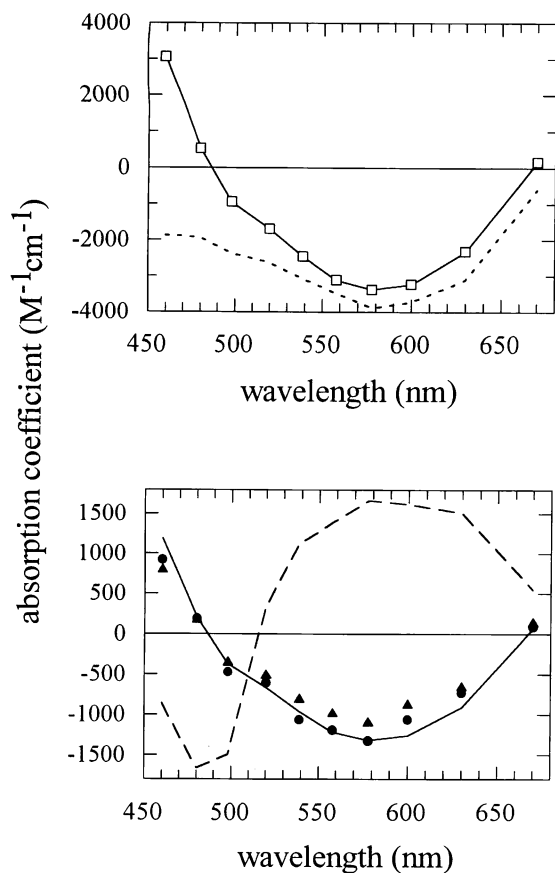
Fig. 2. Simulated and observed OD spectra of PSI-mediated redox transitions of flavodoxin. Upper part: (---) spectrum of the difference (flavodoxin H - - flavodoxin H); (—□—) differential absorption spectrum corresponding to reduction of the semiquinone by [F A /F B ] - , with an absorption decrease being shown as a negative amplitude. Lower part: amplitudes observed at 50 (▲) or 800 μs (●) on signals corresponding to differences between the kinetic traces recorded in the cross-linked and control samples. Absorption coefficients were calculated by reference to the signal observed for P700 + at 820 nm; (—) same spectrum as in the upper part but multiplied by a scaling factor of 0.39; (---) differential absorption spectrum corresponding to the reduction of the oxidized flavodoxin by [F A /F B ] - . Scaling factor, 0.39.
