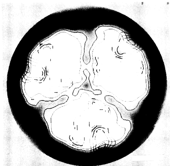
Fig. 8. Scheme for the binding of flavodoxin to PSI, as seen from the cytoplasmic side of the membrane. Indicated by contours are the areas taken by flavodoxin, and the central ridge on the cytoplasmic side of PSI, occupied by the peripheral subunits PsaC, PsaD and PsaE (determined in Kruip et al. , 1993 and J.Kruip, M.Rögner and E.Boekema, unpublished results) superimposed on the image shown in Figure 7b. Scale bar represents 50 Å.
