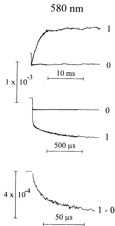
Fig. 5. Flash-induced absorption changes of the photoreduction of the oxidized (upper part) and the semiquinone forms of flavodoxin (middle and lower part) by PSI in solution measured at 580 nm. Both PSI and flavodoxin were obtained from Synechococcus sp. PCC 7002. Experimental conditions: 0.26 \mu\text{M} PSI in 50 mM tricine, pH 8.0, 0.03% \beta -DM, 2 mM sodium ascorbate, 15 \mu\text{M} DPIIP, 5 mM \text{MgCl}_2 and 30 mM NaCl. Traces 0 are control experiments in the absence of flavodoxin; traces 1 are observed in the presence of 20.5 \mu\text{M} flavodoxin. For the reduction of oxidized flavodoxin (upper part), single-flash experiments were recorded after the addition of flavodoxin in complete darkness. Trace 1 corresponds to an average of four different experiments. For recording the reduction of the semiquinone form (middle part), the semiquinone was accumulated by continuous illumination of the samples for 40 s. A series of single-flash experiments was recorded just after the illumination period. The first four flashes exhibited similar kinetics and were subsequently averaged. The lower part shows the difference between a trace recorded in the presence of flavodoxin and a trace recorded in its absence after expansion on a faster timescale. The time of the flash is indicated by a vertical dotted line.
