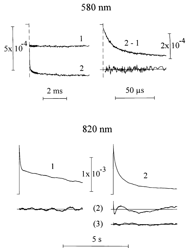
Fig. 1. Flash-induced absorption changes of PSI complexes and PSI complexes cross-linked with flavodoxin at 580 and 820 nm. Experimental conditions: 20 mM tricine, pH 8.0, 2 mM sodium ascorbate, 25 \mu\text{M} DPIP 2 (580 nm) or 1.5 \mu\text{M} DPIP 2 (820 nm), 0.03% \beta -DM, 0.23 \mu\text{M} PSI or PSI–flavodoxin, both from Synechococcus sp. PCC 7002. Band width: DC-1 MHz (580 nm) or DC-30 kHz (820 nm). Repetition rate: one flash every 10 (580 nm) or 60 s (820 nm). Average of 64 (580 nm) or 16 experiments (820 nm). Upper left: trace 1, control (treated EDC); trace 2, PSI–flavodoxin. Upper right: difference between traces 2 and 1 expanded on a 80 \mu\text{s} timescale. A simulated curve is also shown, together with the residuals multiplied by 3. This curve is based on the following parameters: t_{1/2} = 8.9 \mu\text{s} ( 1.88 \times 10^{-4} ), 72 \mu\text{s} ( 0.88 \times 10^{-4} ) and 1.03 ms ( 0.41 \times 10^{-4} ), and includes an offset ( 3.38 \times 10^{-4} ) to take into account longer-lived absorption changes. Lower part: trace 1, control; trace 2, PSI–flavodoxin; Lower traces (2) and (3): corresponding residuals of fits with either two or three exponential components (multiplied by 3). Results of the fits: trace 1, two components, t_{1/2} = 47 \text{ ms} ( 0.75 \times 10^{-3} ) and 4.7 s ( 0.75 \times 10^{-3} ); trace 2, two components, t_{1/2} = 167 \text{ ms} ( 0.98 \times 10^{-3} ) and 2.6 s ( 0.51 \times 10^{-3} ); trace 3, three components, t_{1/2} = 46 \text{ ms} ( 0.37 \times 10^{-3} ), 325 ms ( 0.77 \times 10^{-3} ) and 4.4 s ( 0.34 \times 10^{-3} ).
