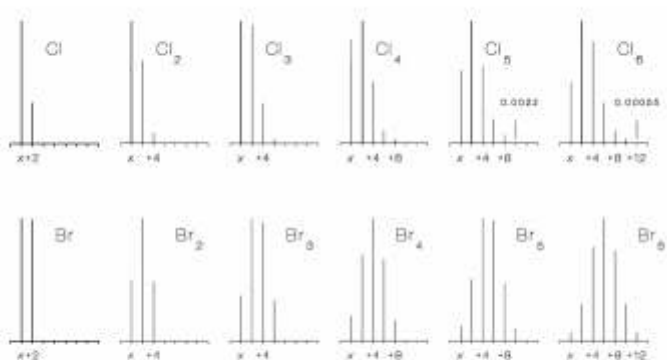
Isotopenmuster
