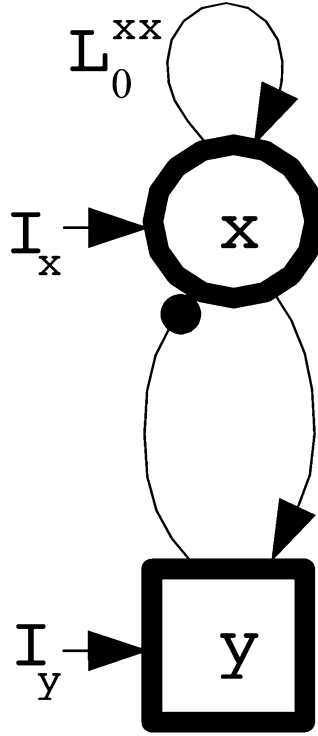
Figure 1a. A single oscillator consists of an excitatory ( x ) and an inhibitory ( y ) neuron. Each neuron represents the average activity of a cluster of biological cells. L_0^{xx} : self-excitation, I_x and I_y : input.
